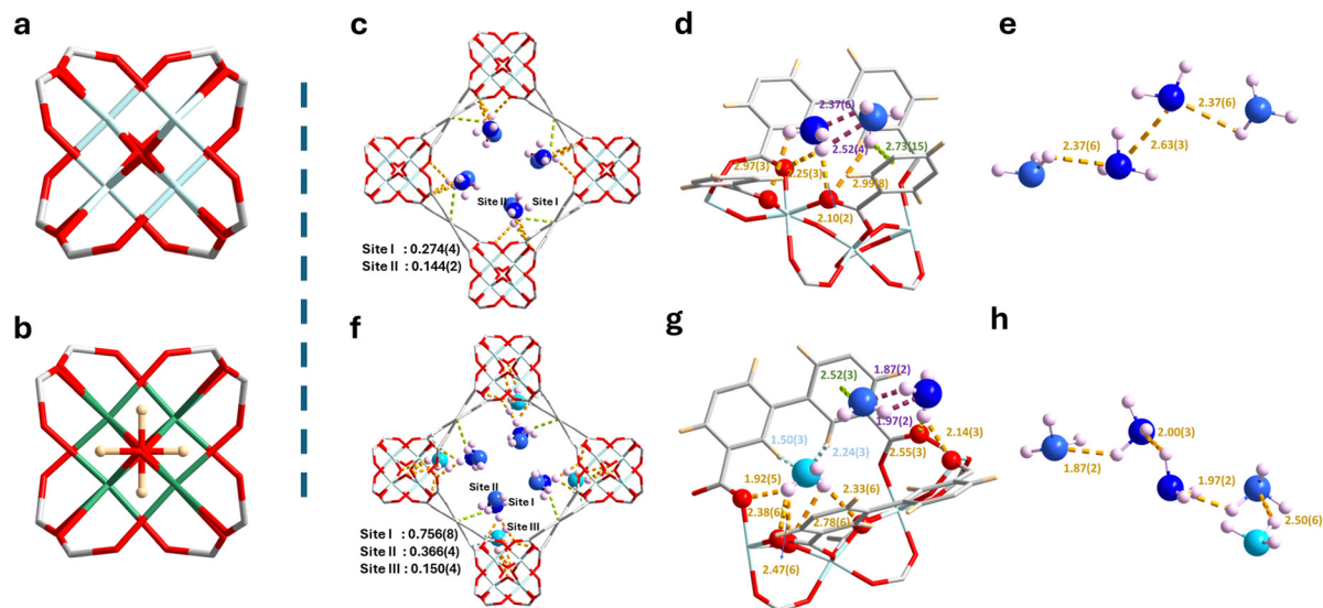
Fig. 1 Views of crystal structures of bare and ND 3 -loaded MFM-300(Ti) as determined by NPD at 10 K. The occupancy of each site has been converted to ND 3 /Ti for clarity. (a) and (b) Views of MFM-300(Ti) and MFM-300(MII) along the c-axis, respectively. (c) and (f) Views of packing of ND 3 in MFM-300(Ti) along the c-axis in MFM-300(Ti)-0.84 ND 3 and MFM-300(Ti)-2.54 ND 3 , respectively. (d) and (g) Detailed views of host-guest interactions in MFM-300(Ti)-0.84 ND 3 and MFM-300(Ti)-2.54 ND 3 , respectively. (e) and (h) Guest-guest interaction along c-axis in MFM-300(Ti)-0.84 ND 3 and MFM-300(Ti)-2.54 ND 3 , respectively. Colour code for atoms: Ti, turquoise; O, red; C, grey; H, tan; N, blue (dark blue, blue, and light blue for site I, II, and III, respectively); D, purple.
