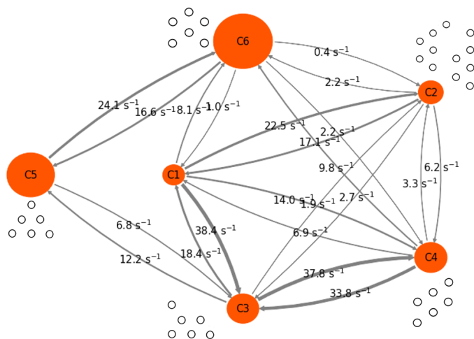
Fig. 4 The state map of the Markov state model (MSM) built for the 6-particle OM system with \tau = 10 ms, n_M = 6 and (beam power, \bar{r} ) = (50 mW, 8.3). The sizes of the orange circles are proportional to the probability distributions of the macrostates. The thickness of the connecting curves is in accord with the magnitude of the transition rates. Representative lattice patterns are shown next to each macrostate; C1 contains a mixture of lattice patterns too numerous to display.
