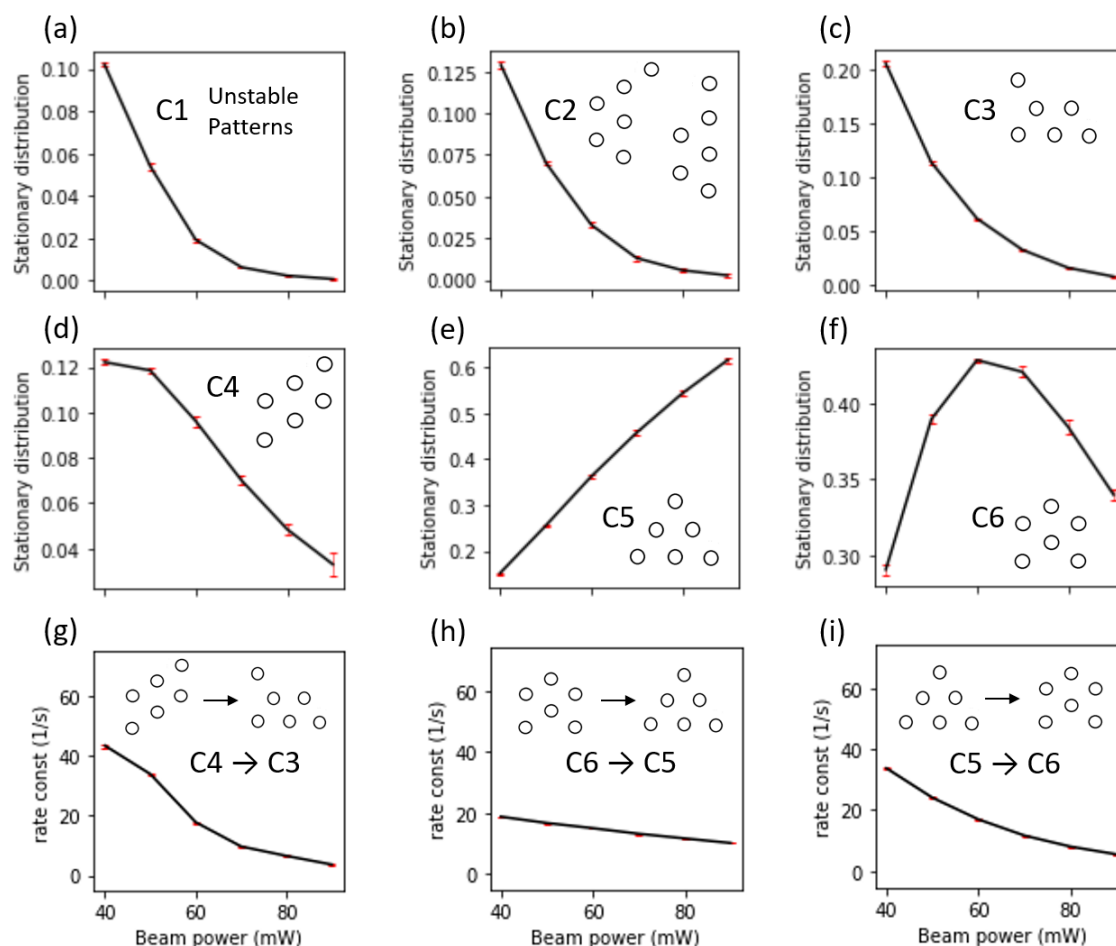
Fig. 5 Plot of (a-f) the stationary distribution probabilities for the six macrostates C1-6 and (g-i) the rate constants of 3 selected macrostate-to-macrostate transitions (C4 → C3, C6 → C5, C5 → C6) as a function of beam power for the 6-particle OM system. Error bars represent standard errors in the mean estimated by five-fold block averaging.
